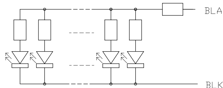
Backlight Circuit (No. of LEDs = 6pcs) Scale=free
