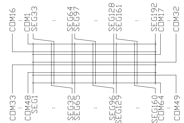
Wiring Details Scale=free
