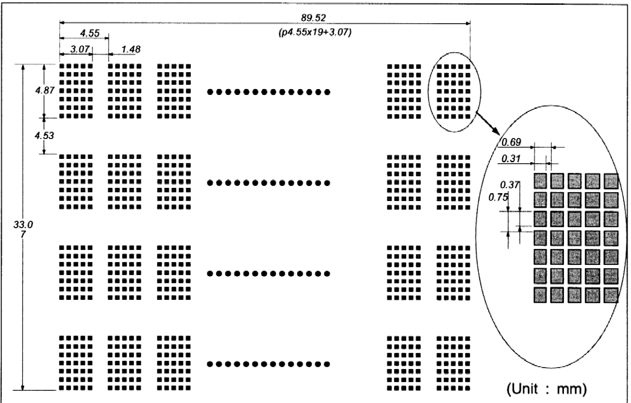
Fig-4. Pattern Details
