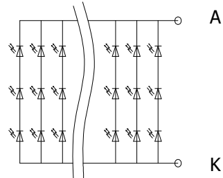
3*8 24LED
